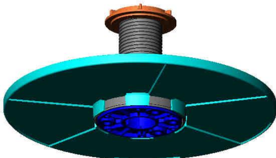
Reel hub assembly type Europa with insulating flange
